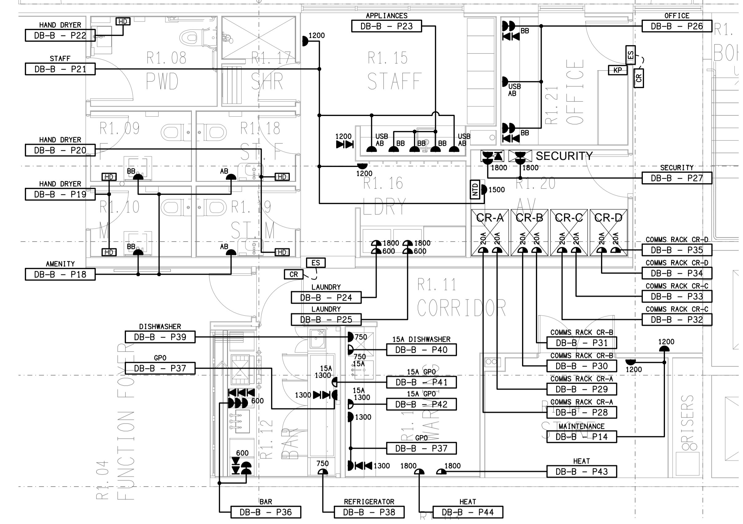
DETAIL A STAFF & BAR LAYOUT SCALE: 1:50
